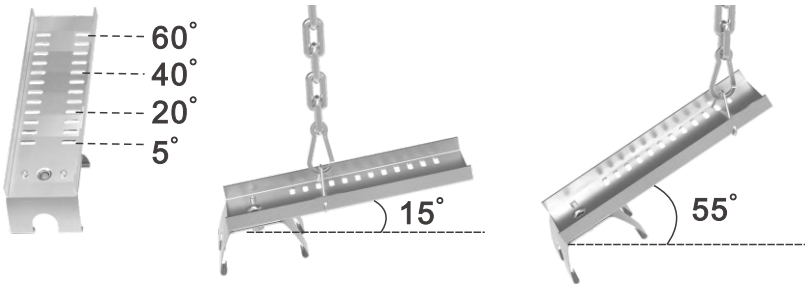
Adjust the angle of the luminaire
